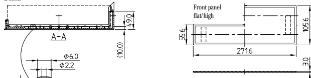
MEDITEC D160 Version II, side trims with ventilation colour lagoon.
