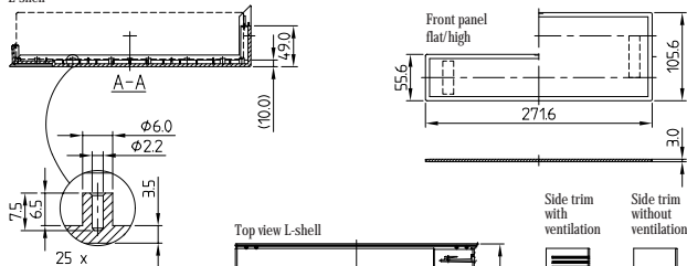
MEDITEC D220 Version II, side trims with ventilation, colour lagoon.
