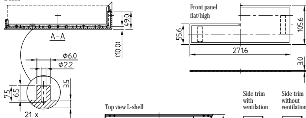
MEDITEC D160 Version II, side trims with ventilation colour lagoon.
