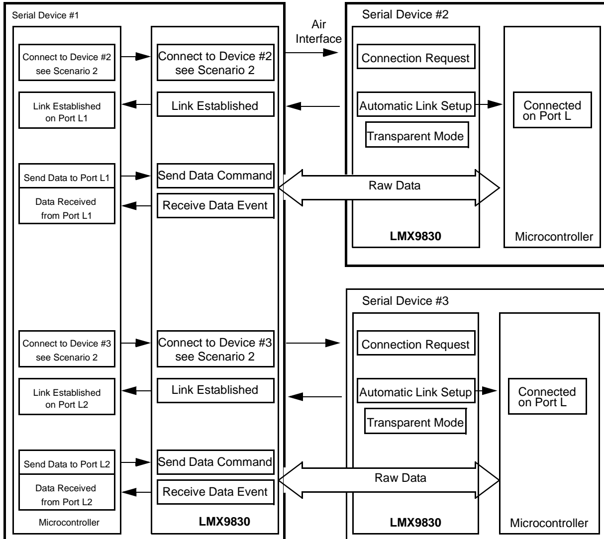
Figure 26. Point-to-Multipoint Connection
