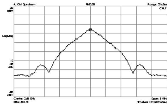
Figure 3. Transmit Spectrum
