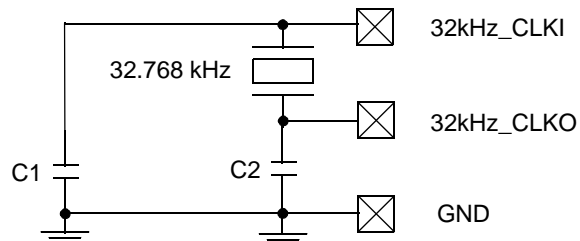
Figure 16. 32.768 kHz Oscillator
